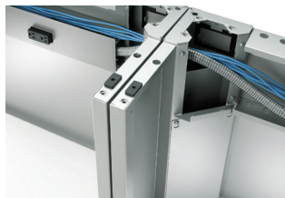
Power and data cleanly pass through leg grommets and efficiently meet at the beltline.
