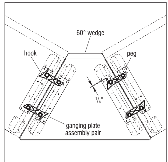
Detail F - 60° Wedge Alignment
