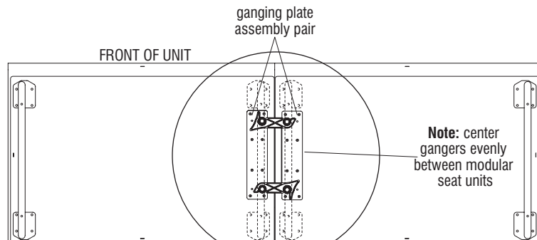
Figure 2 - Bottom View
