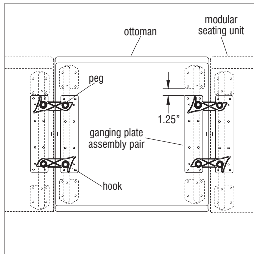
Detail G - Ottoman Alignment
