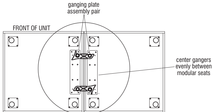
Figure 2 - Bottom View
