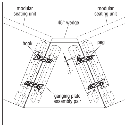
Detail E - 45° Wedge Alignment
