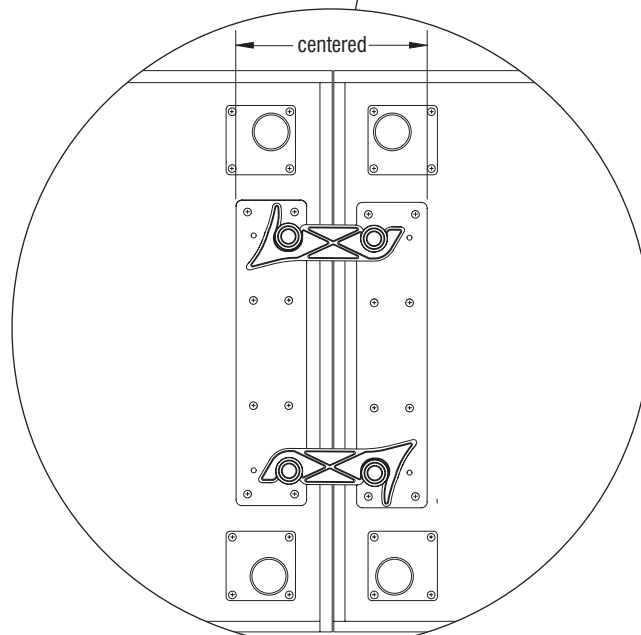
Detail C - Side-to-Side Ganging
