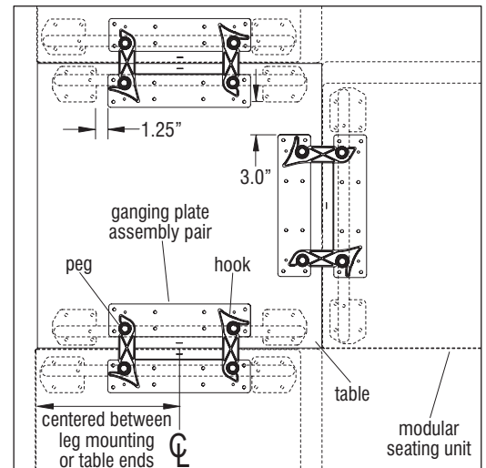
Detail H - Ottoman Alignment
