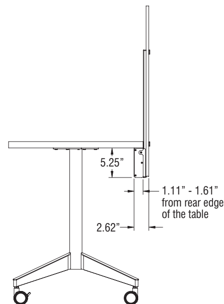
Universal Height-Adjustable Screen - Side View
