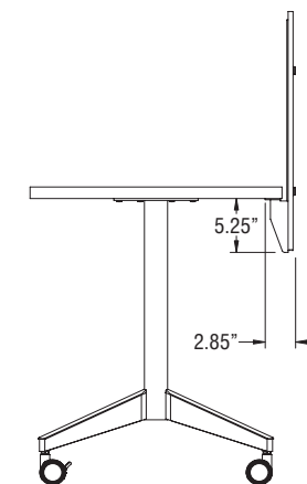
Universal Fixed-Height Privacy Screen - Side View
