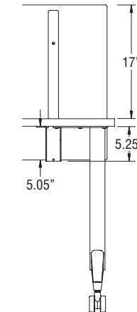
Universal Fixed-Height Privacy Screen - Front View
