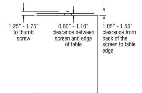
Universal Fixed-Height Privacy Screen - Top View
