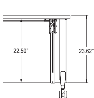
Universal Height-Adjustable Screen - Down Position
