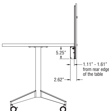
Universal Height-Adjustable Screen - Side View
