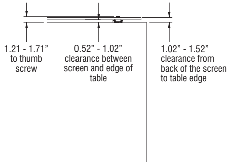
Universal Height-Adjustable Screen - Top View
