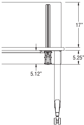
Universal Height-Adjustable Screen - Up Position
