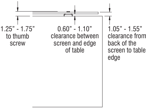
Universal Fixed-Height Privacy Screen - Top View
