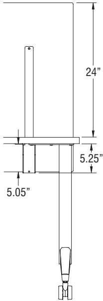
Universal Fixed-Height Privacy Screen - Front View
