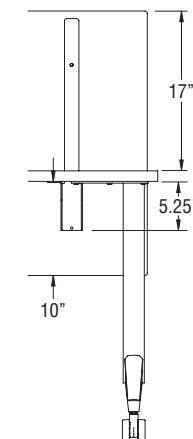
Universal Fixed-Height Privacy Screen & Modesty Panel - Front View
