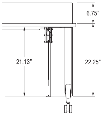
Universal Height-Adjustable Screen - Down Position
