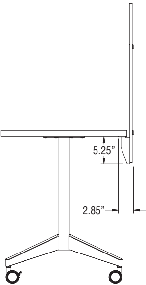
Universal Fixed-Height Privacy Screen - Side View
