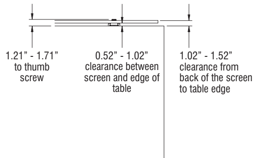
Universal Height-Adjustable Screen - Top View
