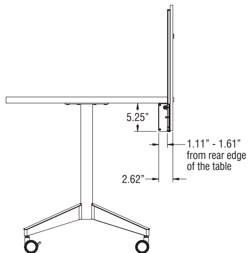
Universal Height-Adjustable Screen - Side View
