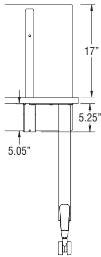
Universal Fixed-Height Privacy Screen - Front View
