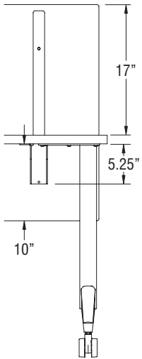
Universal Fixed-Height Privacy Screen & Modesty Panel - Front View
