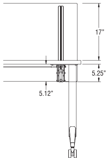
Universal Height-Adjustable Screen - Up Position
