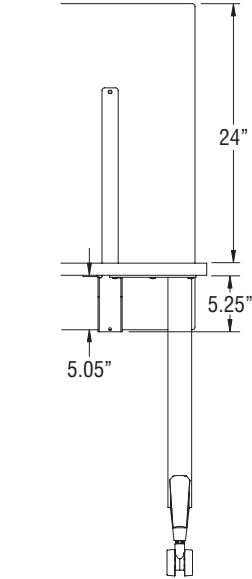
Universal Fixed-Height Privacy Screen - Front View
