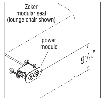
Center-Line Height of Power Module to Floor
