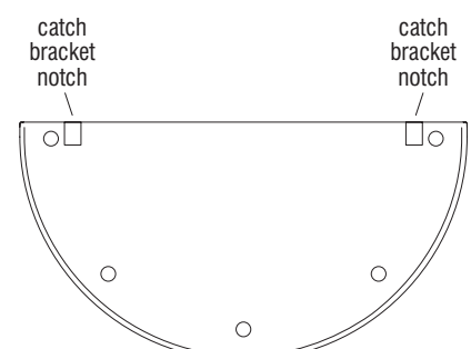
Half Round Ganger Notch Locations (bottom view)
