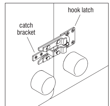
Ganger Kit (engaged)
