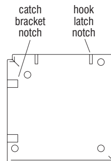
Corner Ganger Notch Locations (bottom view)
