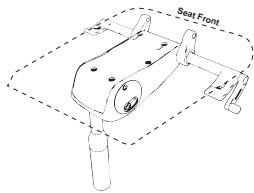
Control Pneumatic synchronous control with seat slider
