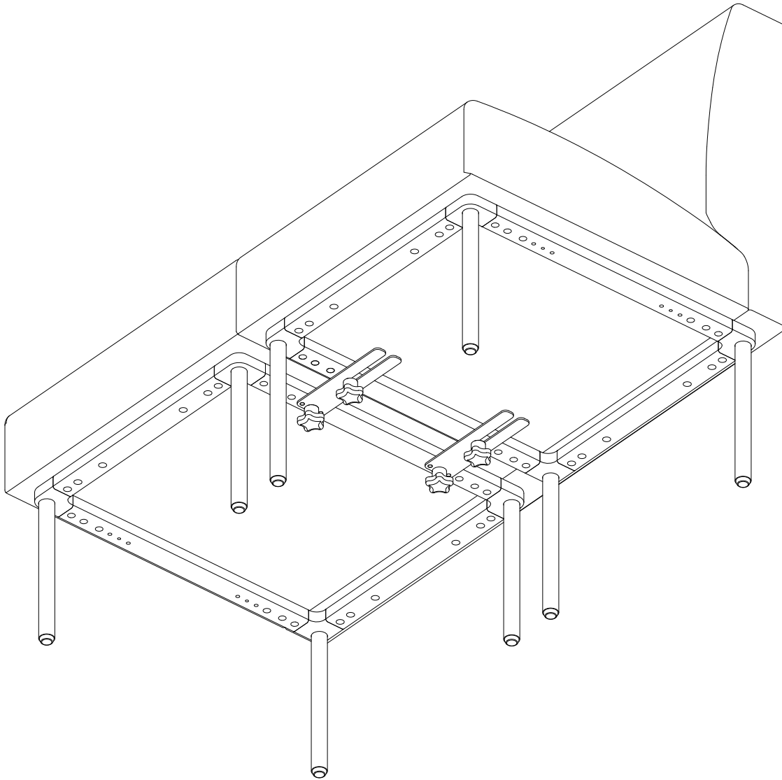
207GK Gangs frames together of freestanding units
