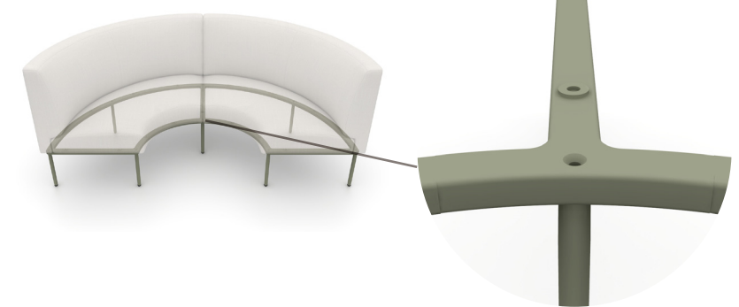
RCCG to LCHG - Outside corner to outside corner connection Outside corner lounge or bench to outside corner lounge or bench
