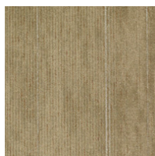
Clay 14150
