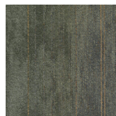
Tourmaline 14320
