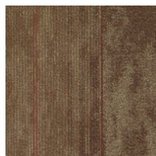
Cinnabar 14713
