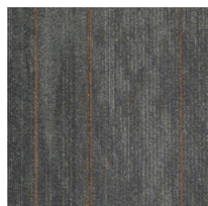
Graphite 14481
