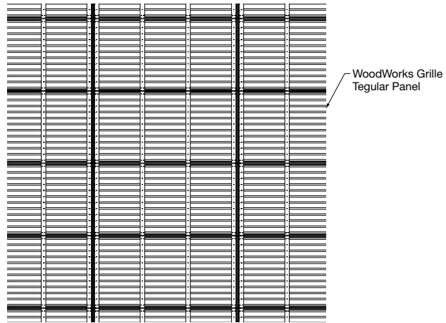
② 6723F51L4T5 Grille Tegular Installation Layout
