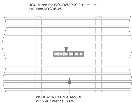
USAI Micro for WOODWORKS – Vertical Slats Fixture Housing
