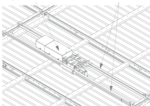
USAI Micro for WOODWORKS – Vertical Slats Fixture Housing
