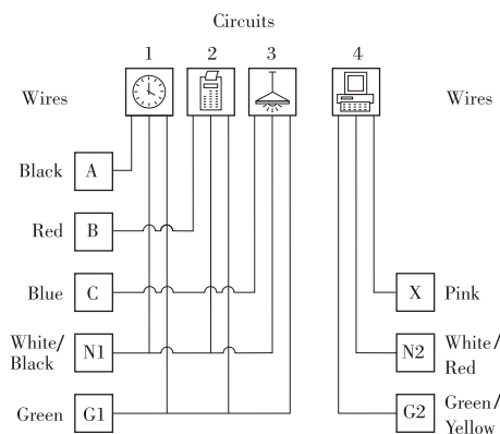
Wiring Diagram (3+1)
