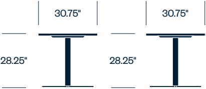
Small Square Collaborative Table with 4-Star Base, Aluminum Slat Top
