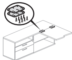
Convergent Bracket
