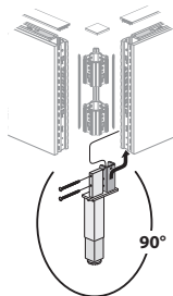
Glass Panel without Raceway Cover
