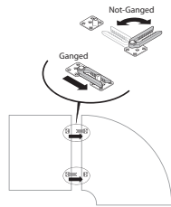
Ganging Bracket
