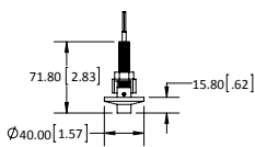
(P2) MONOPOINT DIA. 1.6" W/ THREADED NIPPLE MOUNTING
