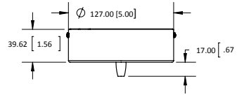
(E4) MONOPOINT 5" CANOPY W/ &+-+V BALLAST OR LED 277V/12V TRANSFORMER
