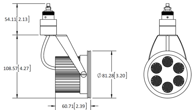
DIMENSIONS ARE IN MILLIMETERS [INCHES] (NOT TO SCALE)
