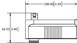
(27) H-TRACK ADAPTER
