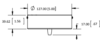
(E3) MONOPOINT 5" CANOPY W/ 120V BALLAST OR LED 120V/12V TRANSFORMER
