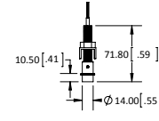
(P1) MONOPOINT DIA. 0.7" W/ THREADED NIPPLE MOUNTING
