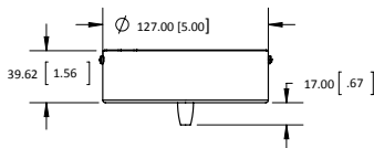
(E4) MONOPOINT 5" CANOPY W/ BALLAST OR LED 277V/12V TRANSFORMER
