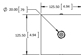
(P4) 5" DIRECT MOUNT SQUARE COVER PLATE
