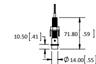
(P1) MONOPOINT DIA. 0.7" W/ THREADED NIPPLE MOUNTING
