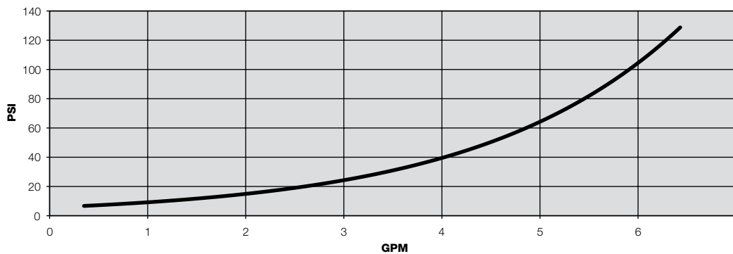
Figure 1. Flow Capacity: Pressure vs. GPM
