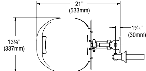
Dust Cover
