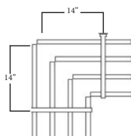
Exterior Mitred Corners
