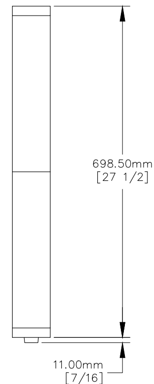
RIGHT VIEW
