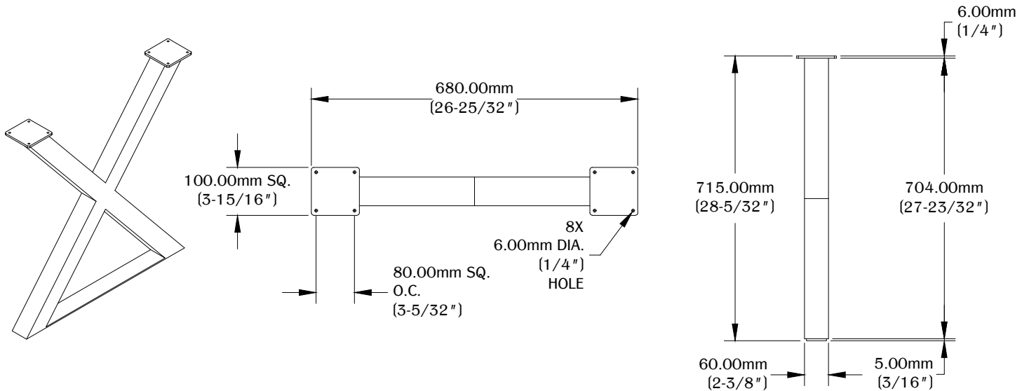
TOP VIEW
