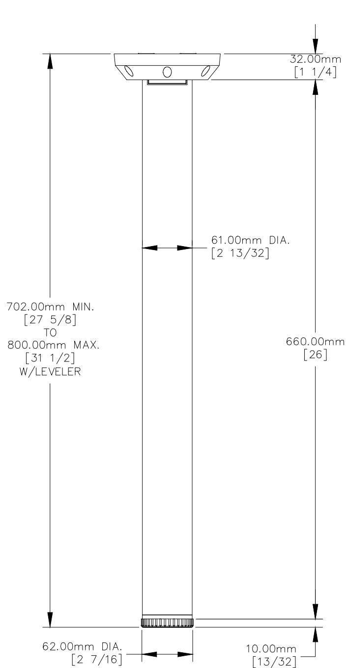
FRONT VIEW
