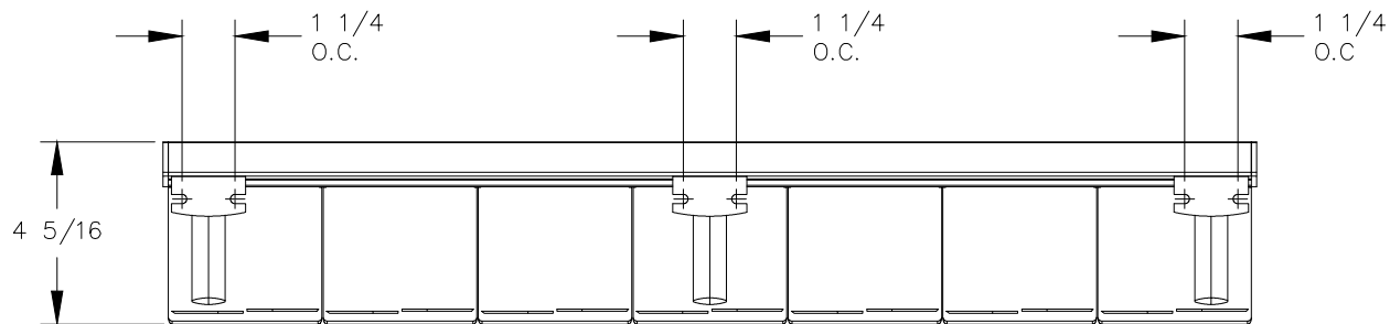
TOP VIEW
