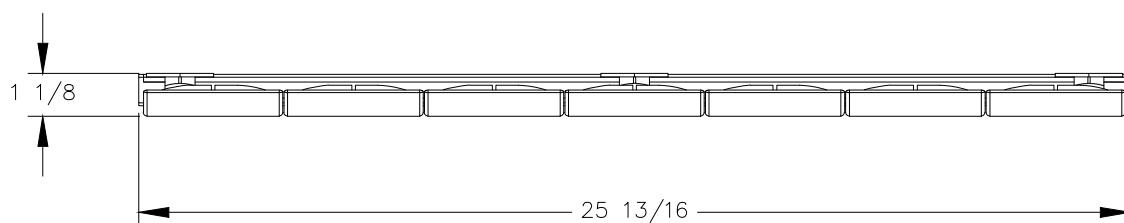
FRONT VIEW
