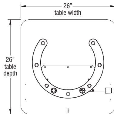
Square Table CMDGC26 (26" Fixed-Height) CMDAC26 (29" Fixed-Height) CMDEC26 (Adjustable-Height)
