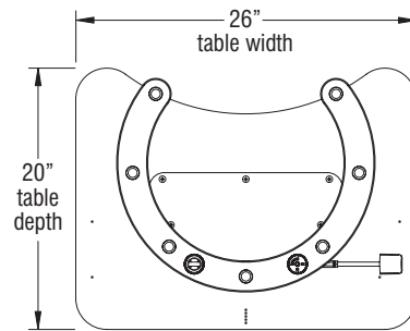
20" x 26" Rectangular Table with Comfort Curve CMDGN2026 (26" Fixed-Height) CMDAN2026 (29" Fixed-Height) CMDEN2026 (Adjustable-Height)
