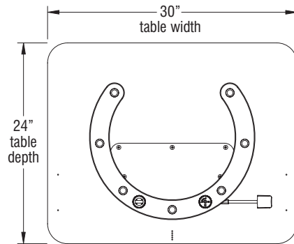
24" x 30" Rectangular Table CMDGA2430 (26" Fixed-Height) CMDAA2430 (29" Fixed-Height) CMDEA2430 (Adjustable-Height)
