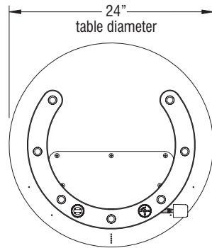
Round Table CMDGB24 (26" Fixed-Height) CMDAB24 (29" Fixed-Height) CMDEB24 (Adjustable-Height)
