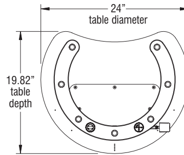
Round Table with Comfort Curve CMDGP24 (26" Fixed-Height) CMDAP24 (29" Fixed-Height) CMDEP24 (Adjustable-Height)
