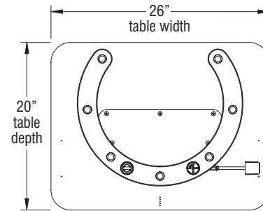
20" x 26" Rectangular Table CMDGA2026 (26" Fixed-Height) CMDAA2026 (29" Fixed-Height) CMDEA2026 (Adjustable-Height)
