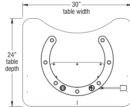
24" x 30" Rectangular Table with Comfort Curve CMDGN2430 (26" Fixed-Height) CMDAN2430 (29" Fixed-Height) CMDEN2430 (Adjustable-Height)
