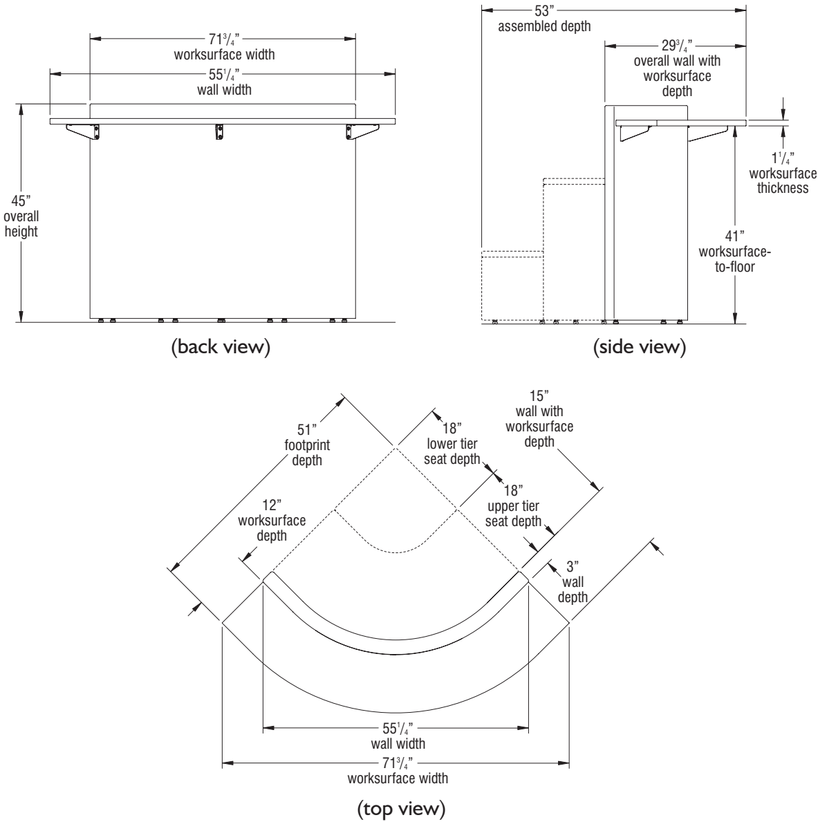
Clamber Wall - Inside Corner - (model CLSCNN & CLAWSN-74P shown below)
