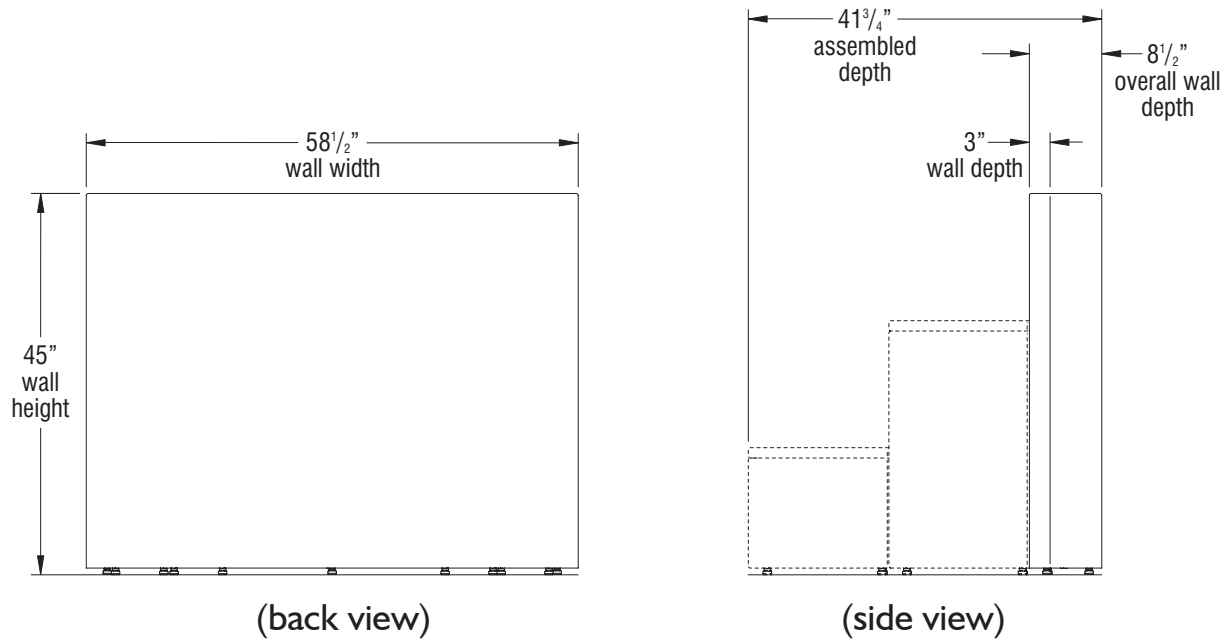
Clamber Wall - Inside Curve - 45 Degree - (model CLWVN shown below)
