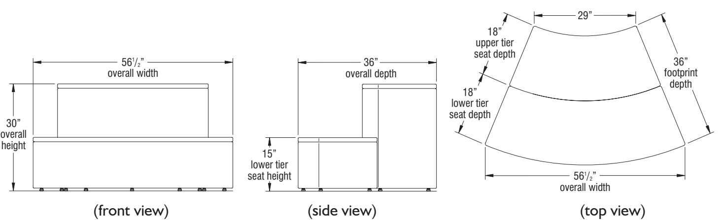
Clamber Two-Tiered Seating - Outside Curve - 45 Degree - (model CL2VT shown below)
