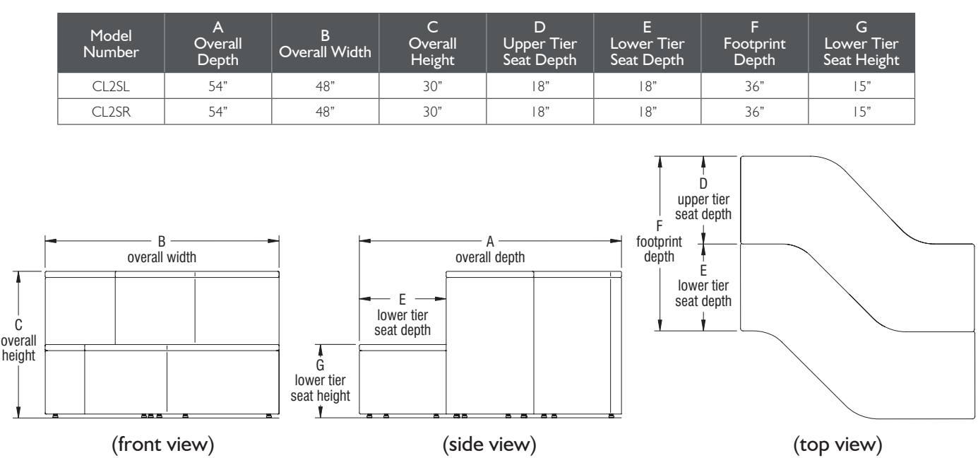
Clamber Two-Tiered Seating - S-Curve - (model CL2SL shown below)
