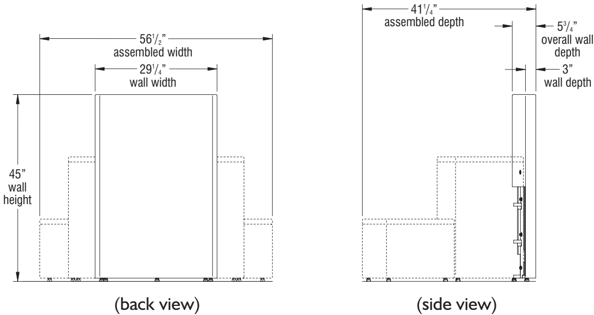
Clamber Wall - Outside Curve - 45 Degree - (model CLWVTN shown below)
