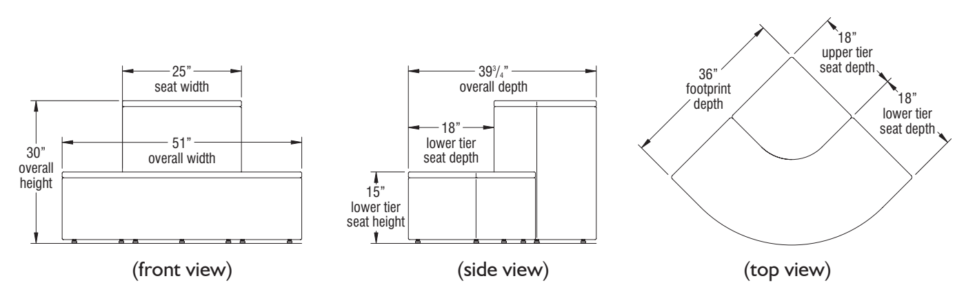
Clamber Two-Tiered Seating - Outside Corner - (model CL2CT shown below)
