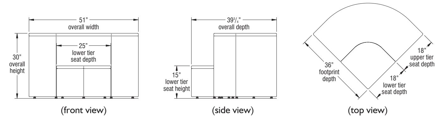
Clamber Two-Tiered Seating - Inside Corner - (model CL2CN shown below)
