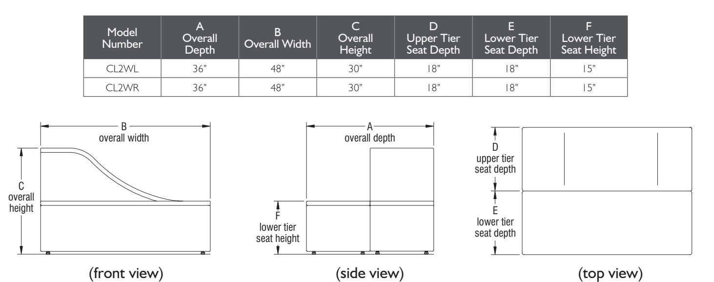
Clamber Two-Tiered Seating - Wave - (model CL2WL shown below)
