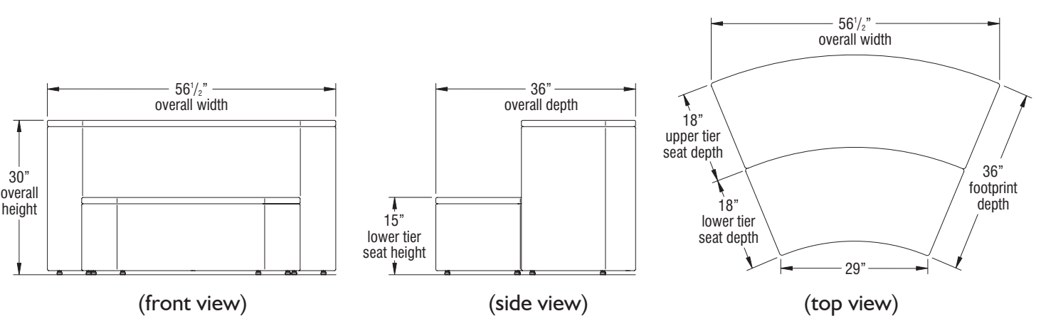
Clamber Two-Tiered Seating - Inside Curve - 45 Degree - (model CL2VN shown below)
