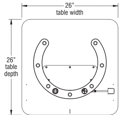
Square Table CMDGC26 (26" Fixed-Height) CMDAC26 (29" Fixed-Height) CMDEC26 (Adjustable-Height)
