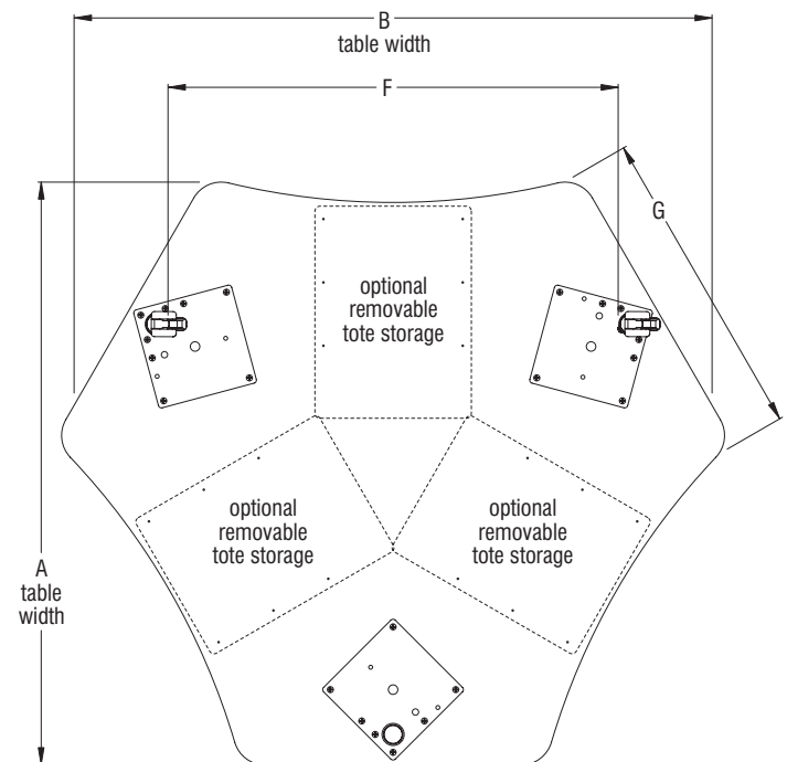
Sprocket Table - 20"-24" (bottom view)
