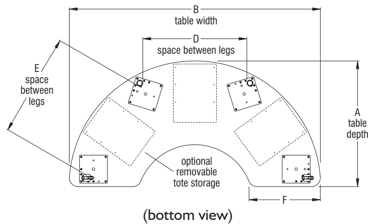
(model RTEEF367220 with caster/glide base shown)
