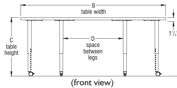
(model RTEEF367220 with caster/glide base shown)
