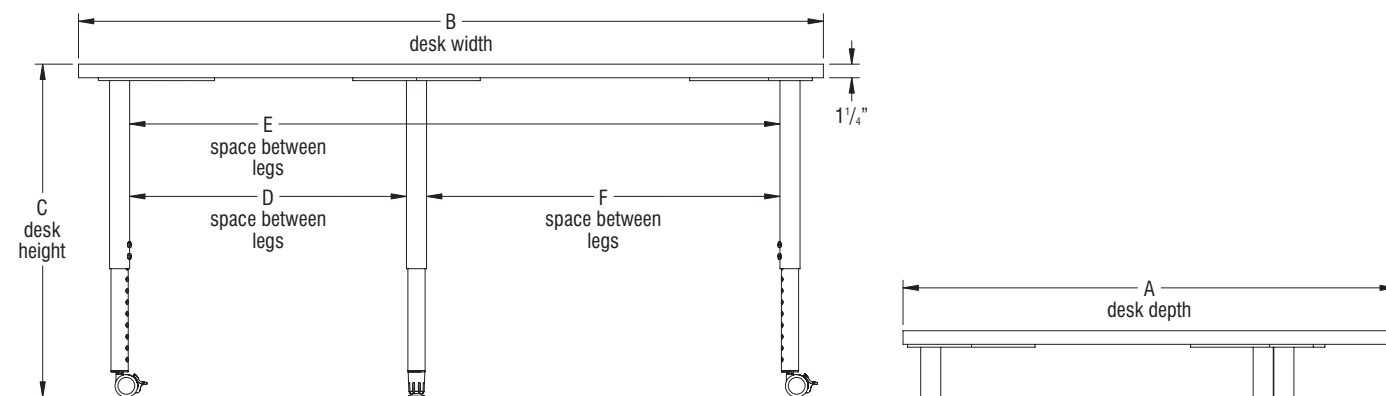
(front view)
