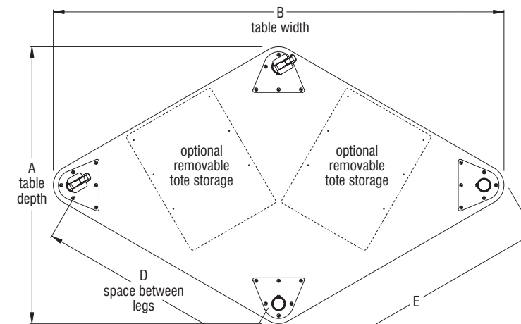
(bottom view)
