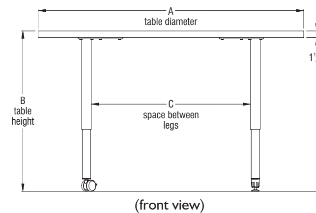
(model RTEEB48 with caster/glide base shown)
