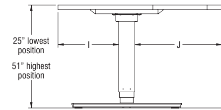
120° Corner Dual Motor T-Leg Electric-Base Table
