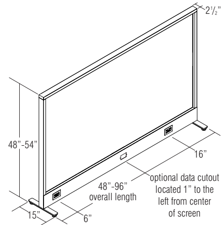
Spine Screen with Hardwired Electrical (Chicago Code) & Data
