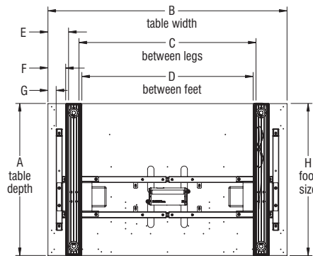
Rectangular Dual Motor C-Leg Electric-Base Table
