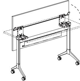
TJJMA Rectangle Table w/Single Circuit - 24"D
