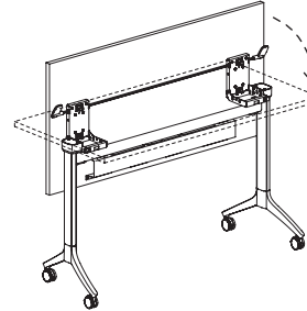
TJJMA Rectangle Table w/Single Circuit - 30"D
