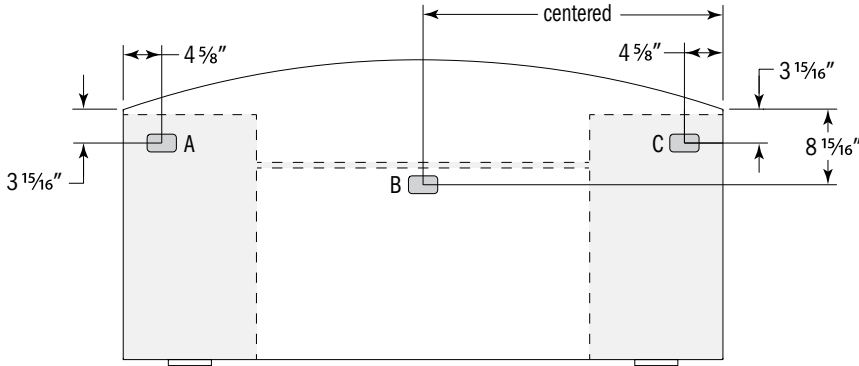
Desks without Overhangs (Bow Front Shown)
