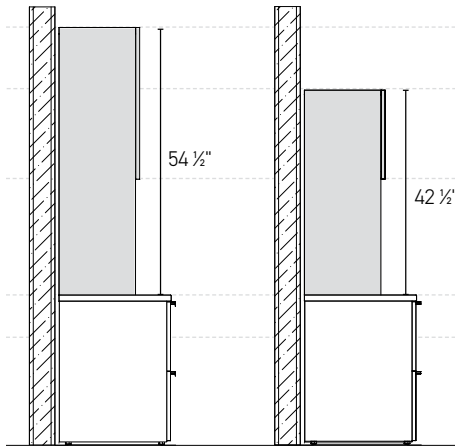
54 ½" overhead cabinet with standard height credenza
