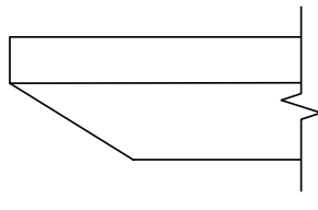
Reverse Bevel (K9) PVC on painted top of painted MDF
