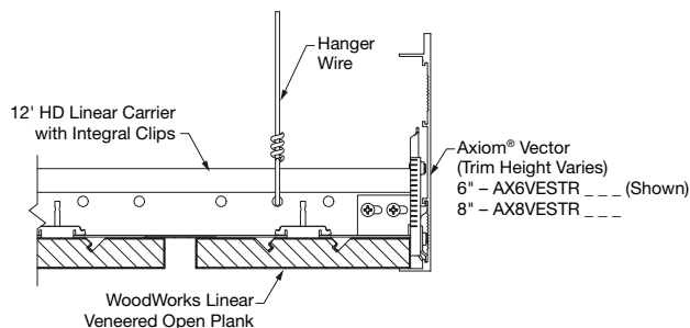
3 Axiom® Perimeter Trim
