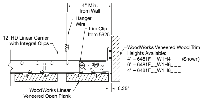
4 Veneered Perimeter Trim
