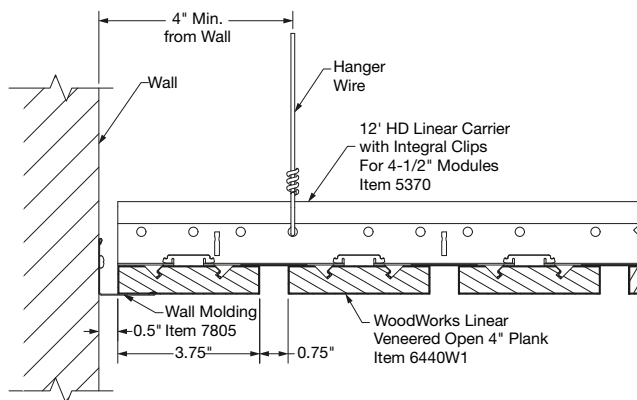
2 Linear Veneered Open Wall Perimeter Detail
