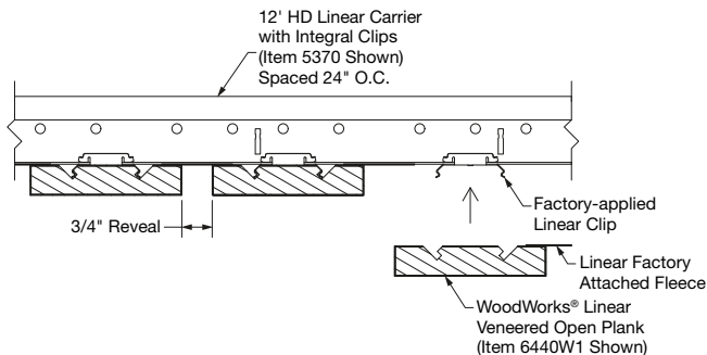
1 Linear Veneered Open Plank to Grid Install
