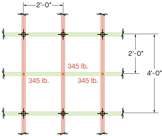
4' × 2' Support Spacing Main Beam Mid-Span Loading
