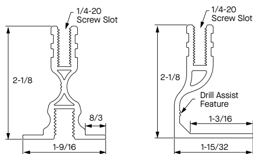
DynaMax LT Main Beam
