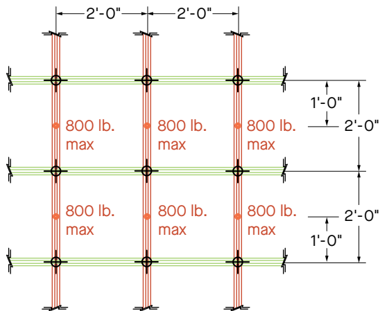
2' × 2' Support Spacing Main Beam Mid-Span Loading
