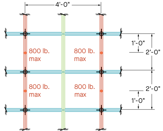
2' × 4' Support Spacing Main Beam Mid-Span Loading
