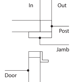
Plan view of T-post
