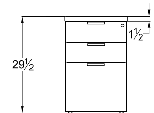
Pedestal Front Profile Box/Box/File
