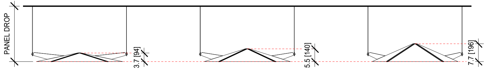
SECTION VIEW OF 36" PANELS
