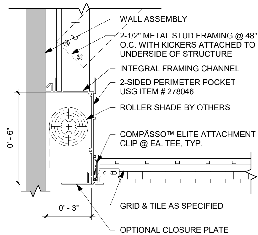
ACOUSTICAL FLANGE / INTEGRAL FRAMING CHANNEL ② 2-SIDED CURTAIN POCKET DETAIL 3" = 1'-0"
