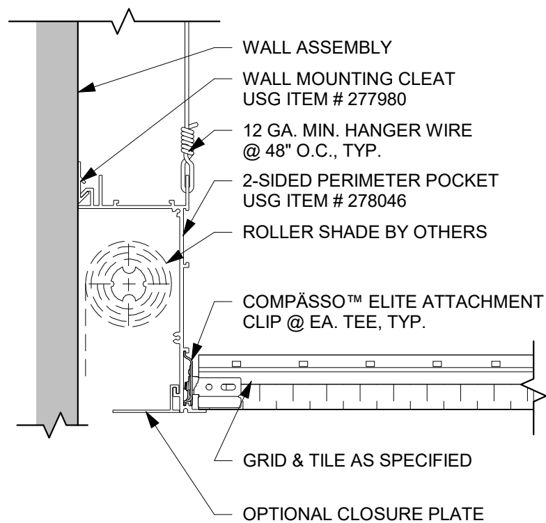
ACOUSTICAL FLANGE / INTEGRAL FRAMING CHANNEL ① 2-SIDED CURTAIN POCKET DETAIL 3" = 1'-0"
