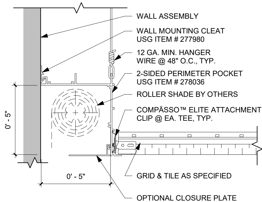
1 ACOUSTICAL FLANGE / INTEGRAL FRAMING CHANNEL 2-SIDED CURTAIN POCKET DETAIL 3" = 1'-0"
