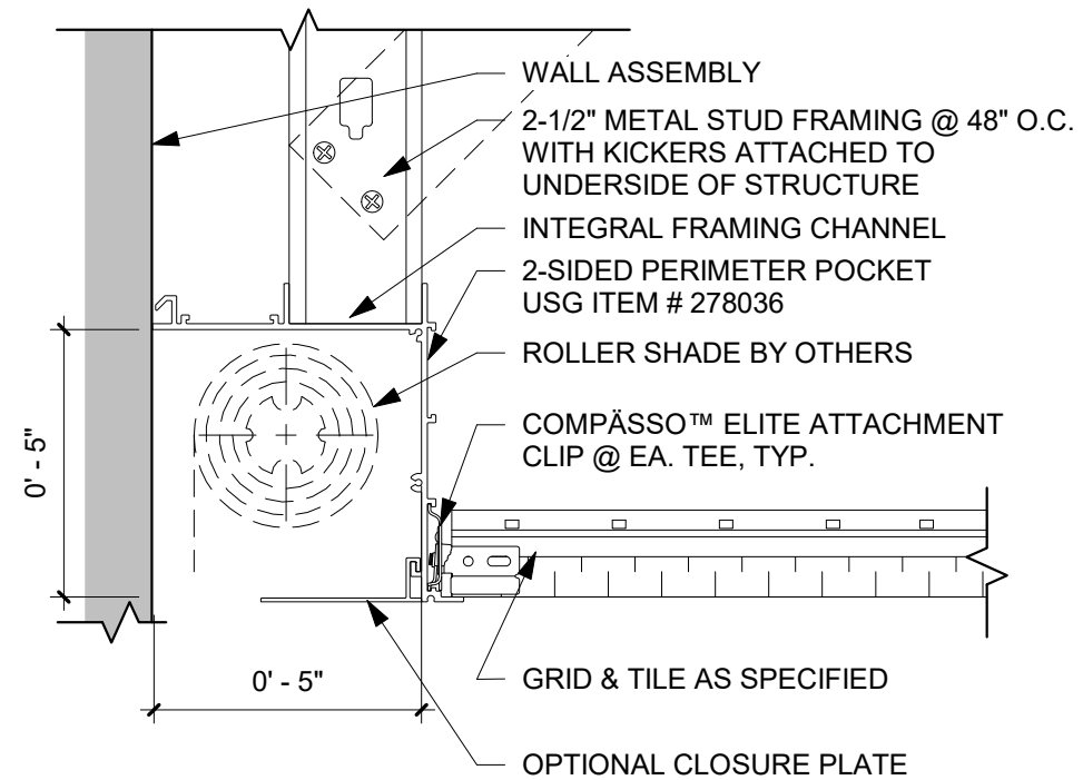
2 ACOUSTICAL FLANGE / INTEGRAL FRAMING CHANNEL 2-SIDED CURTAIN POCKET DETAIL 3" = 1'-0"
