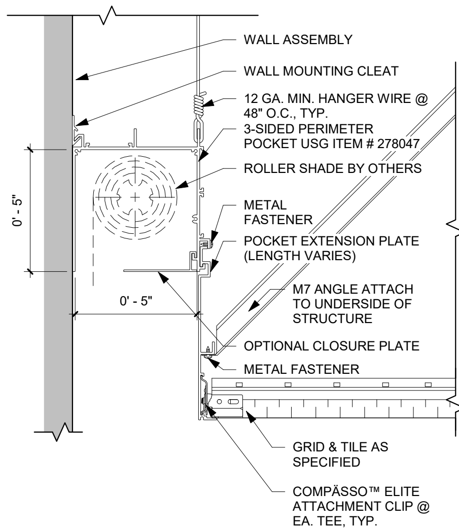
1 ACCOUSTICAL FLANGE / INTEGRAL FRAMING CHANNEL 3-SIDED CURTAIN POCKET DETAIL 3" = 1'-0"
