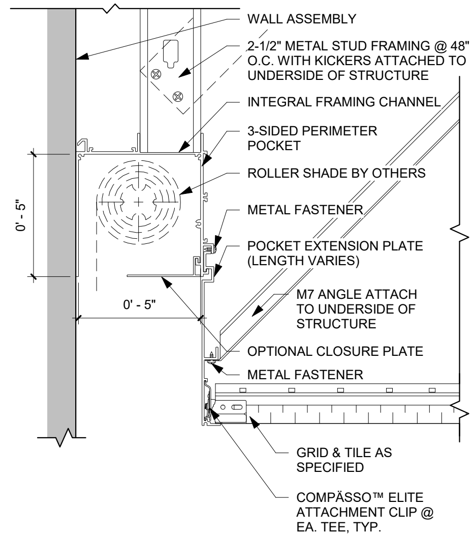
2 ACCOUSTICAL FLANGE / INTEGRAL FRAMING CHANNEL 3-SIDED CURTAIN POCKET DETAIL 3" = 1'-0"
