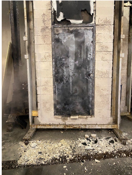
Figure 16: The exposed side of assembly 2 after the hose stream test.
