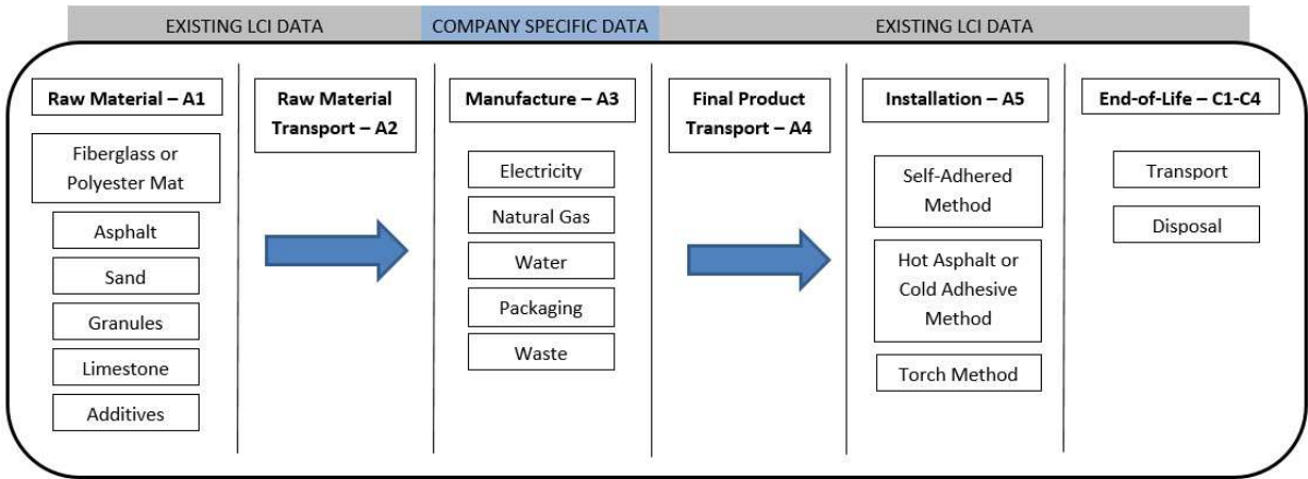
Figure 2: BUR Non-Modified Asphalt Commercial Roofing Product Flow Diagram
