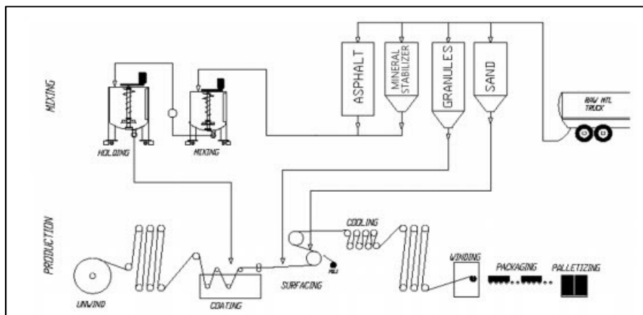
Figure 3: Manufacture of Commercial Roofing Products
