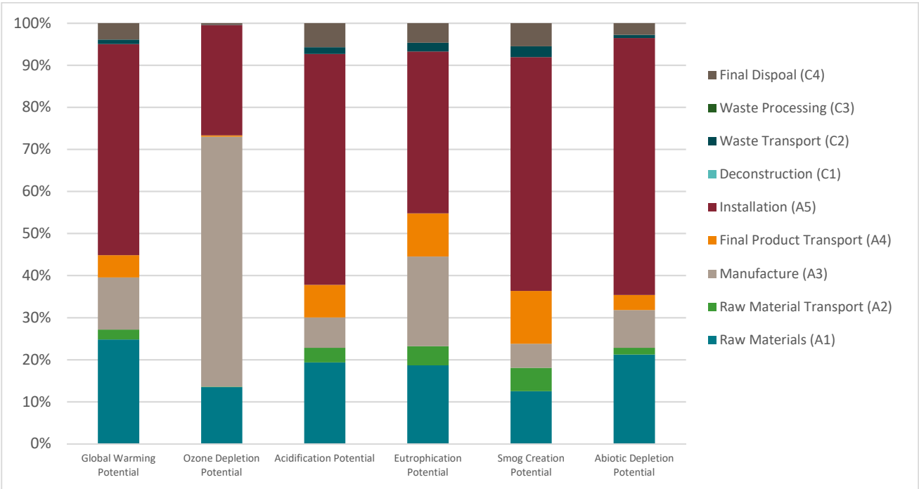
Figure 5: BUR Non-Modified Asphalt Cap Sheets TRACI 2.1 Environmental Impacts
