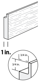
Built-in J-Pocket for siding
