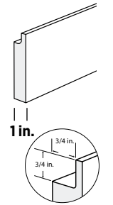
Built-in J-Pocket for siding
