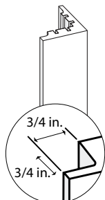
Built-in J-Pocket for siding
