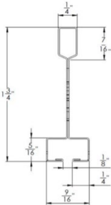
9/16" Bolt Slot Grid Profile 1/8" (8EZB)
