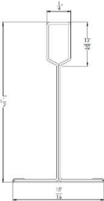
15/16" EZ Stab Classic Grid Profile (EZCS) and 15/16" EZ Torsion Spring Grid Profile (EZTS)
