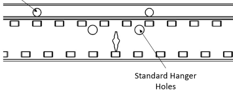
FIGURE 15—EZ HANGER HOLE LOCATIONS
