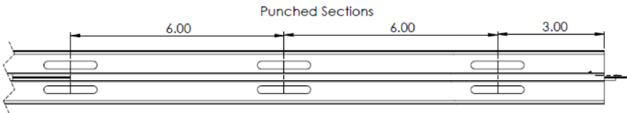
Flange Slots for TSW
