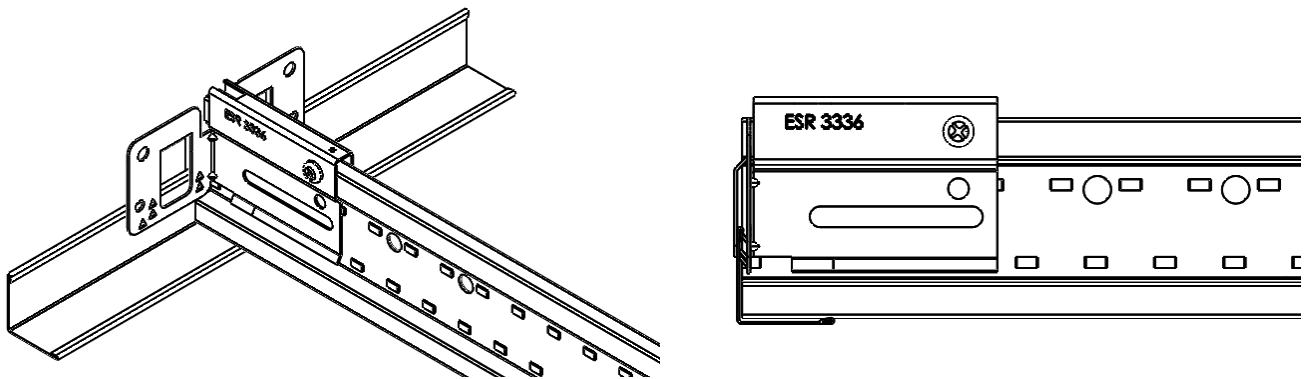
FIGURE 11 — 9/16" EZ STAB BOLT SLOTS AND 9/16" EZ STAB TIER DROP FIXED WALL SETUP WITH WALL ANGLE (WA14-14) AND SEISMIC PERIMETER CLIP (SEISMIC DESIGN CATEGORIES A, B, C, D, E AND F) IN SECTIONS 4.2.3 AND 4.2.5
