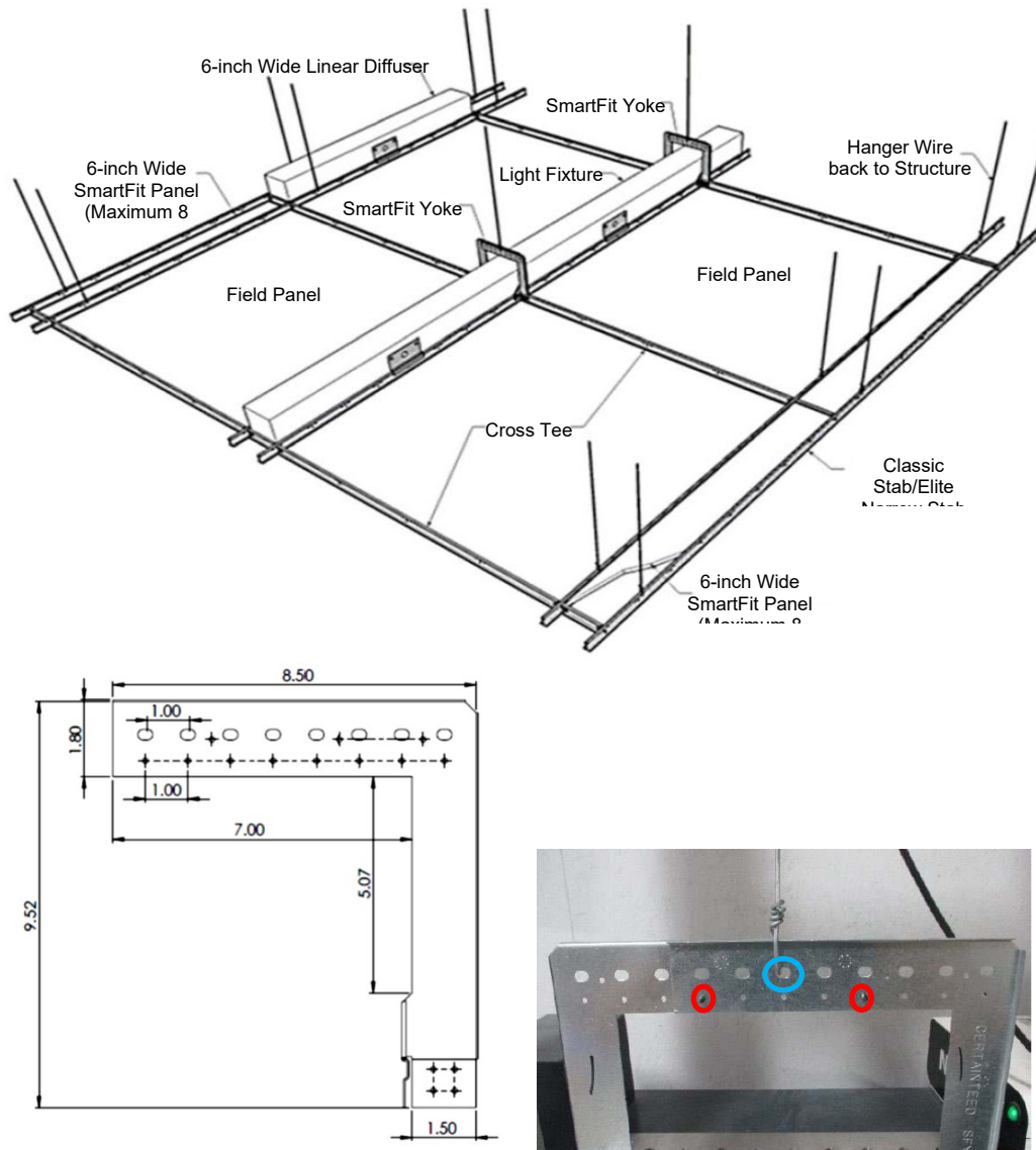
FIGURE 19—SMARTFIT YOKE SYSTEM (SFYK)
