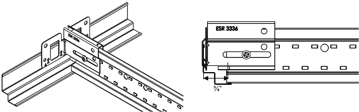
FIGURE 10 — 9/16" EZ STAB BOLT SLOTS AND 9/16" EZ STAB TIER DROP FREE WALL SETUP (LOOSELY SCREWED) WITH SHADOW MOLD (SM1020, SM1040 OR SM1050) AND SEISMIC PERIMETER CLIP (SEISMIC DESIGN CATEGORIES D, E AND F) IN SECTION 4.2.3
