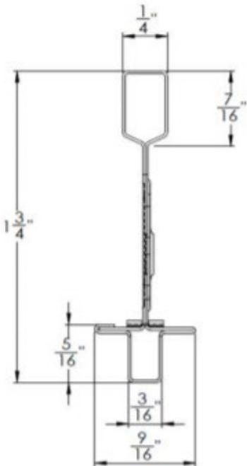
Tier Drop Grid Profile (EZTD)
