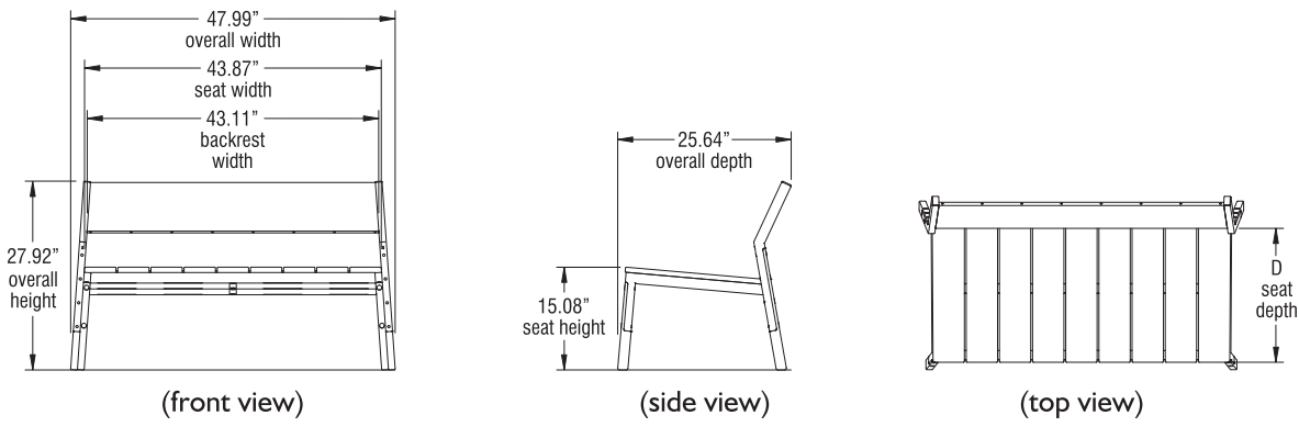
Outspan Lounge Sofa - (model OSFBS shown)
