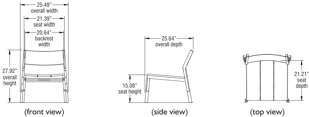
Outspan Lounge Chair - (model OSCBS shown)
