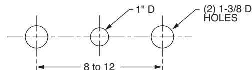
DECK MOUNTING HOLES
