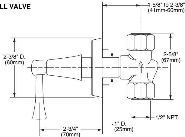
3/4" WALL VALVE
