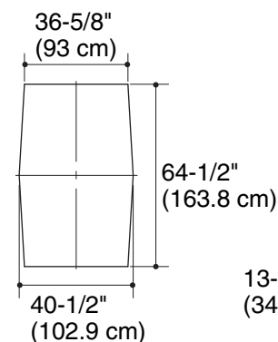
Cut-out Detail
