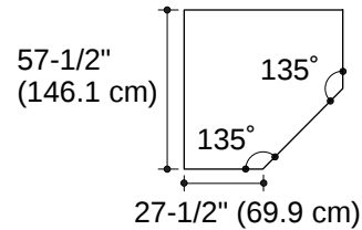
Drop-In Rim Style Cut-Out Detail
