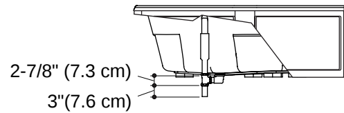
Drop-In Rim Style Cut-Out Detail
