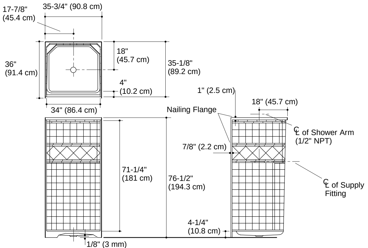
Product Diagram
