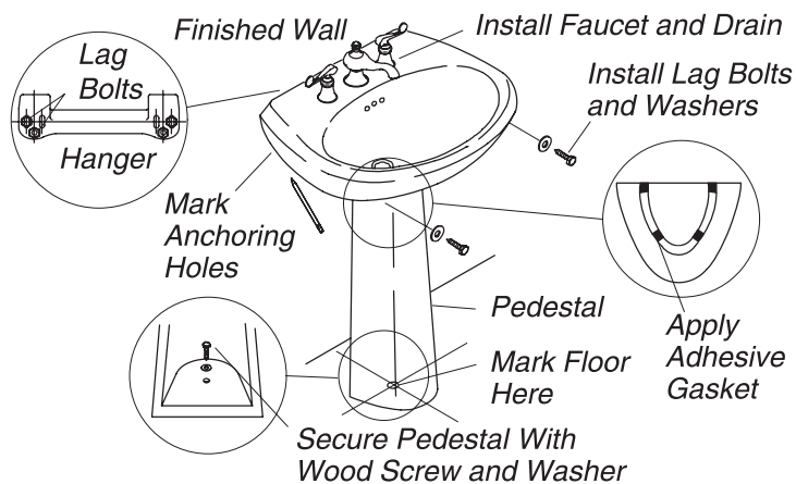
Pedestal and Lavatory Placement
