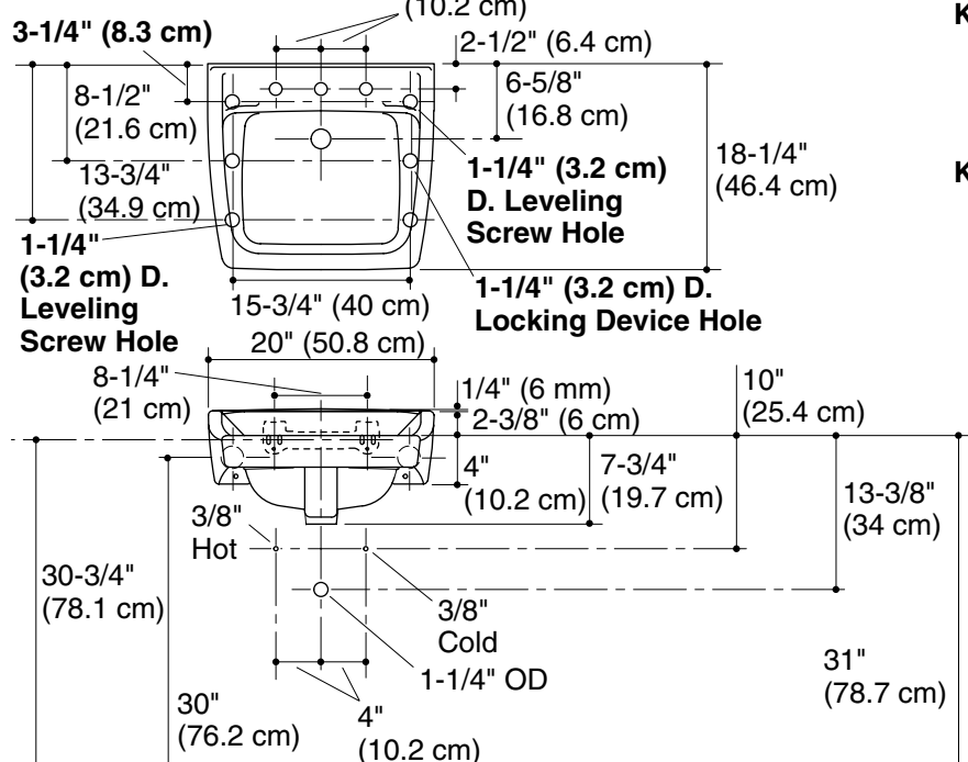
Standard Installation
