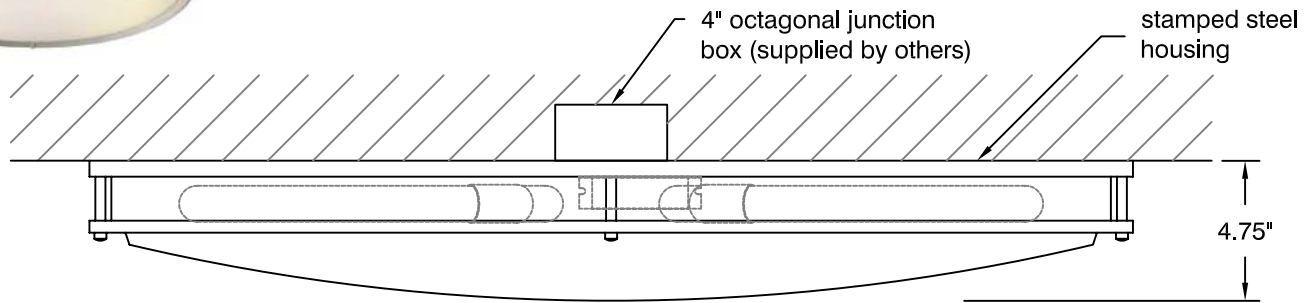
SIDE VIEW
