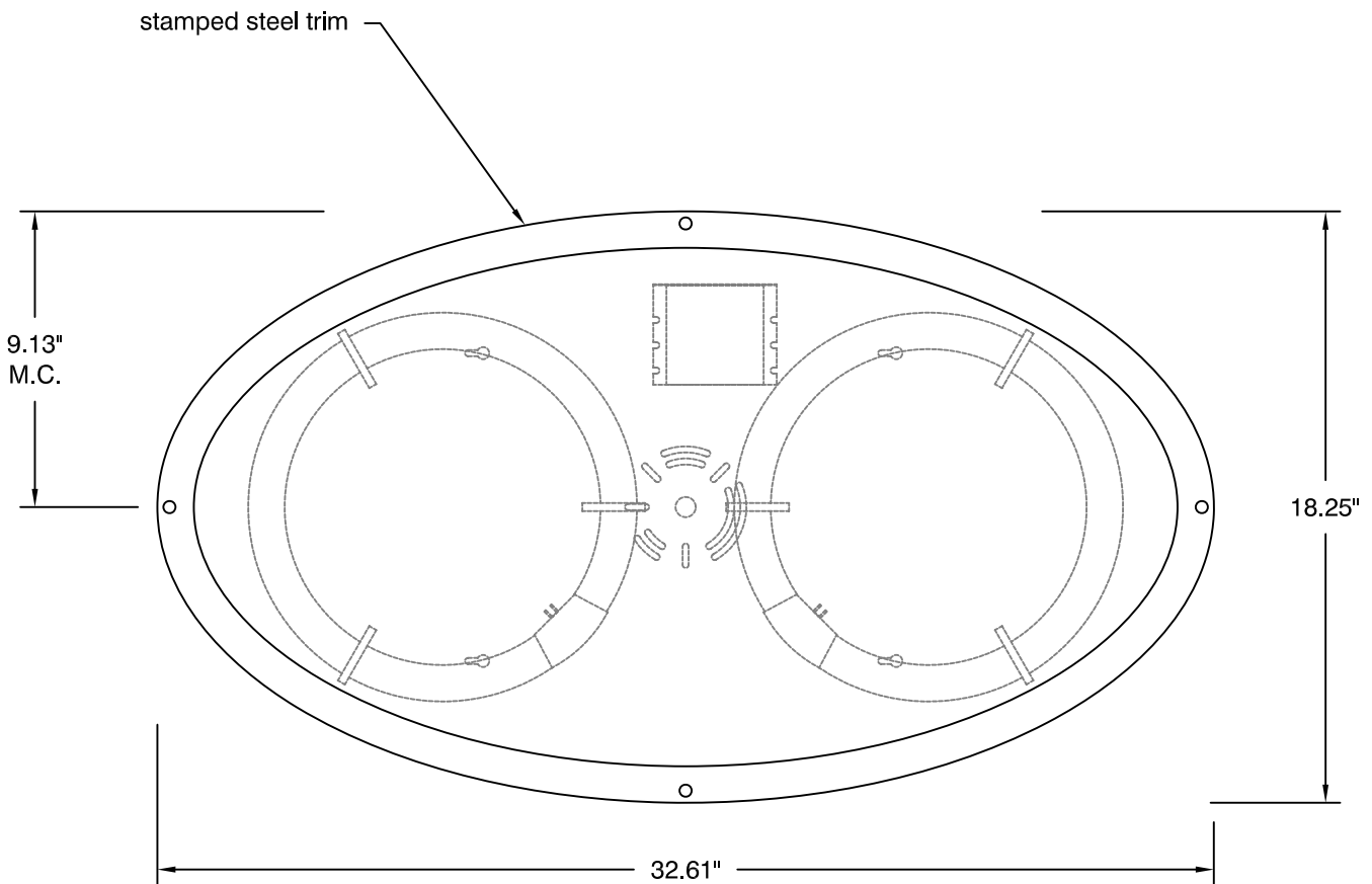
BOTTOM VIEW
