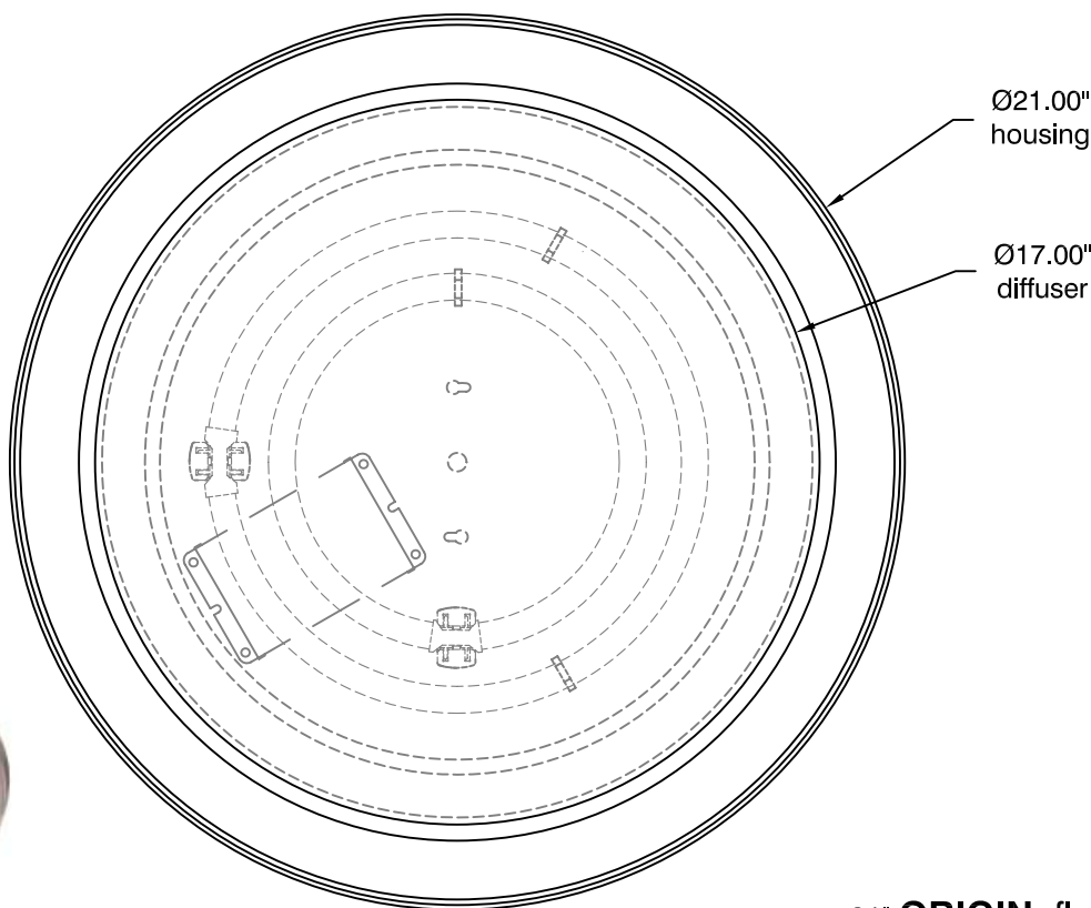
BOTTOM VIEW
